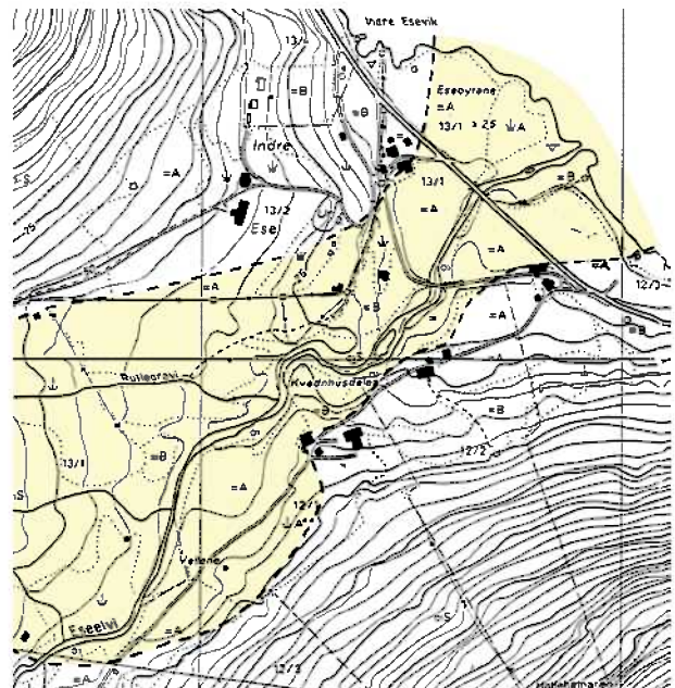
Fig. 2 Esei, Balestrand, West Norway, 09.02.1928 a) Map scale 1: 50 000 show a huge basin with numerous creeks feeding water into an area where slab avalanches can trigger slushflows. Slushflows may also be released in the basin without impact by avalanche. b) Map scale 1:10 000 with the runout zone of the slushflow of 1928. The annals have information on large slushflows during the 1900 th century which reflects the location of the farms. To-day, there is a pressure on building industry as well as recreational homes on the delta by the fiord.
